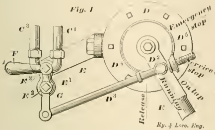
SAND BLOWER AND BRAKE ATTACHMENT.
